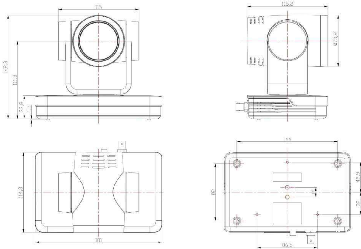
Figure 2.1 Camera dimension
